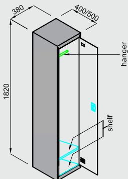
1 DOOR LOCKER CABINET
