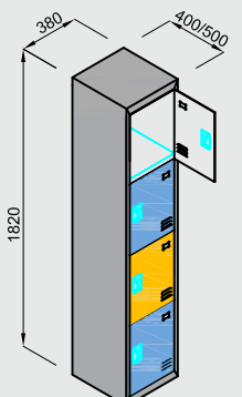
4 DOOR LOCKER CABINET
