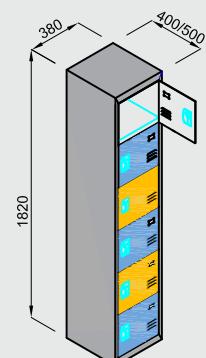
6 DOOR LOCKER CABINET
