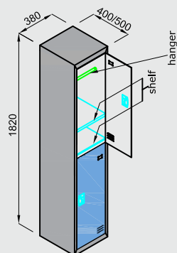
2 DOOR LOCKER CABINET
